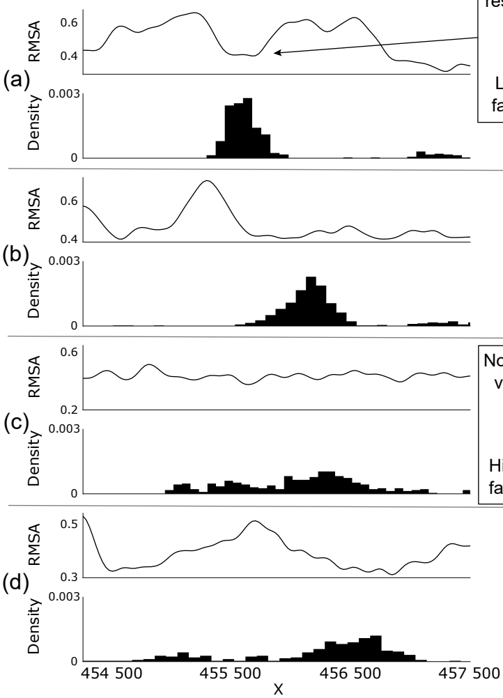
Y-averaged rms amplitude of boxes
