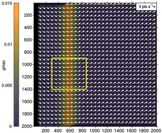
(a) Vector field + maximum shear
