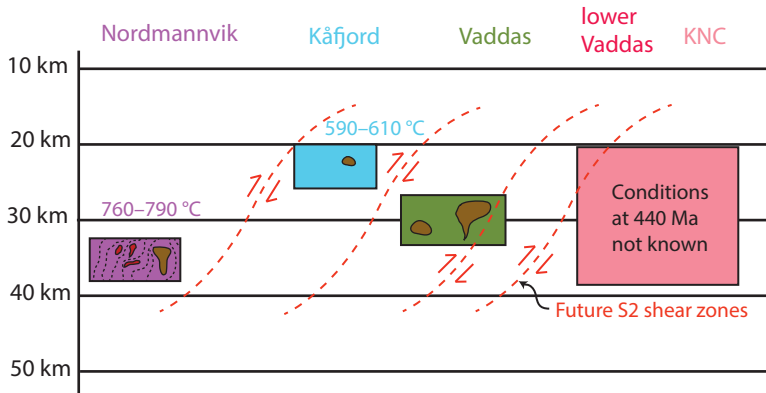
(b) Relative position of nappes during D_2 shearing (440–430 Ma)
