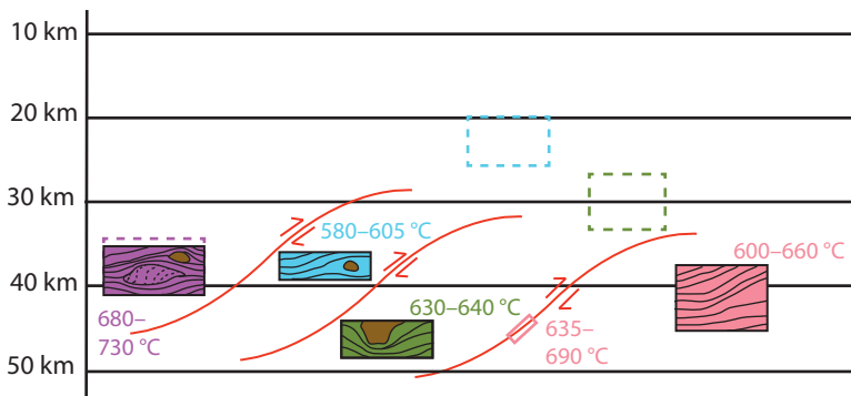
(b) Relative position of nappes during D_2 shearing (440–430 Ma)
