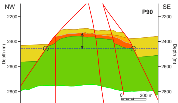
(a) Section D-D'
