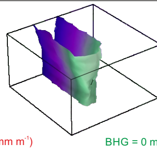
(f) Permeability anisotropy = 10 2 N-S oriented
