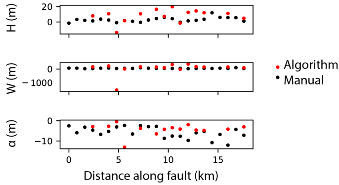
Figure S17. Top: The misfit analysis for the southern Malombe fault (SMAF). Bottom: The misfit between manual analysis and algorithm using the best performing parameters for twenty-five selected profiles.
