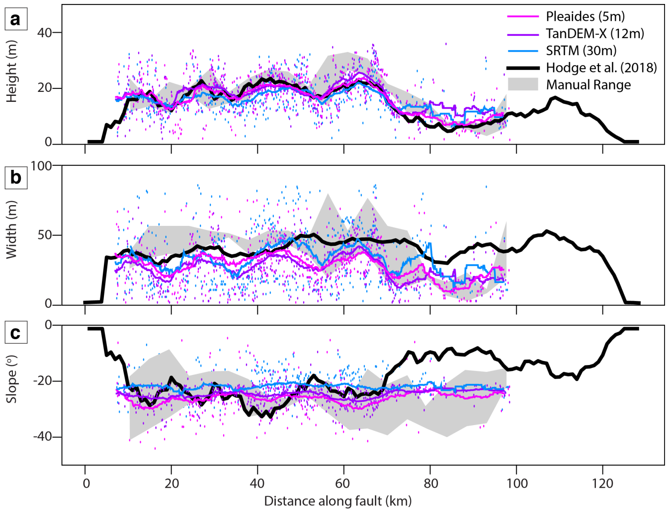
Figure S11. The quality checked height, width and slope profiles using the algorithm on Pleiades 5 m (pink), TanDEM-X 12 m (purple) and SRTM 30 m (blue) DEMs. A moving mean (window size of 7 km) is shown by a solid line coloured corresponding to the DEM used. The manually derived TanDEM-X moving mean (window size of 7 km) from Hodge et al. (2018) is shown by a black line and the envelope of manual DEM results in this study is shown by the grey polygon.
