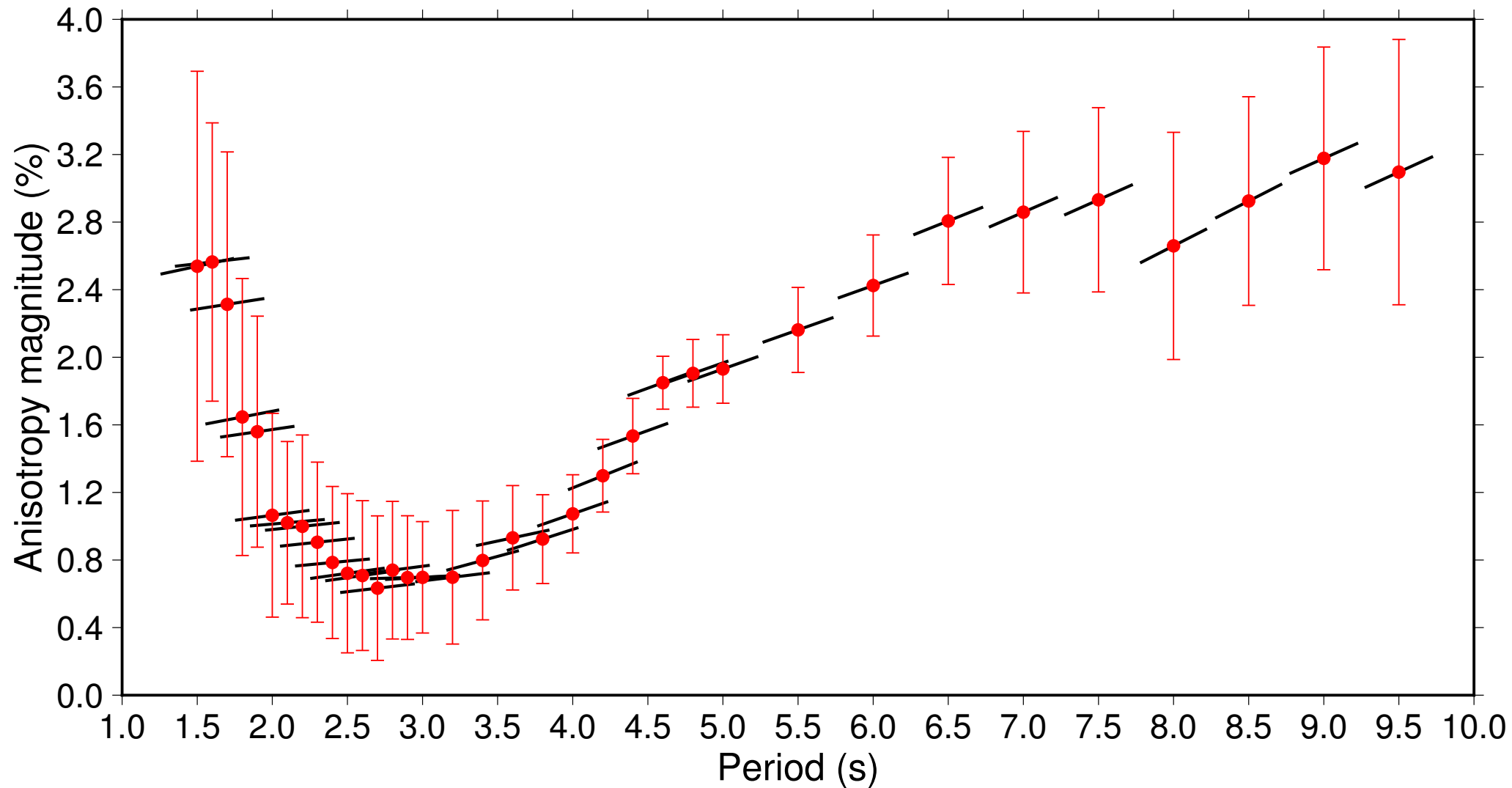
Variation of Rayleigh wave anisotropy with period
