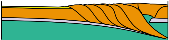
Short thin- and thick-skinned thrust sheets
