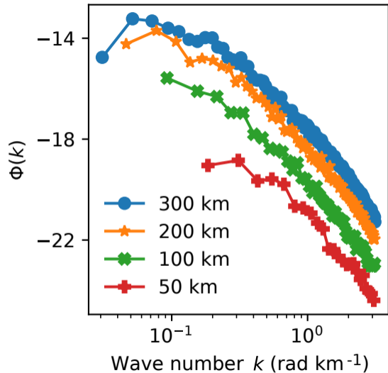
(b) Radial power spectrum
