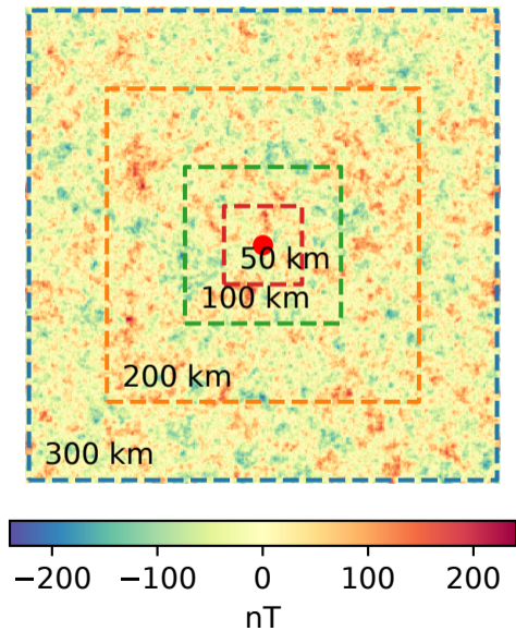
(a) Magnetic anomaly
