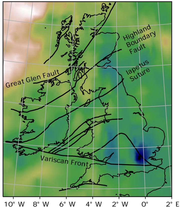
(b) Crustal thickness
