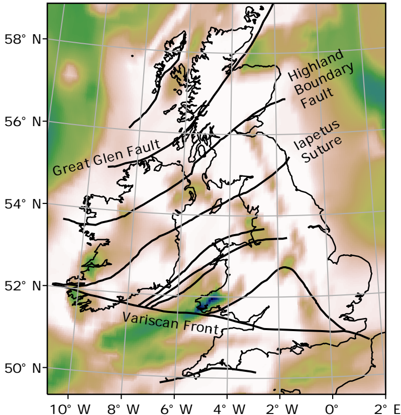
(a) Sedimentary thickness
