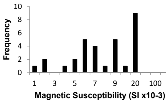
Thaduna Formation n=32
