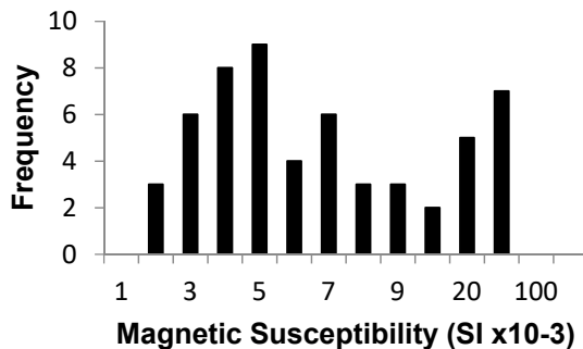
Killara Formation n=56
