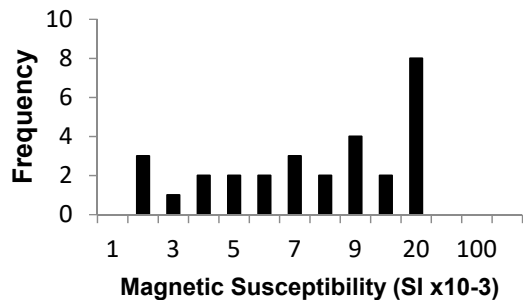
Micro-gabbroic dyke n=30
