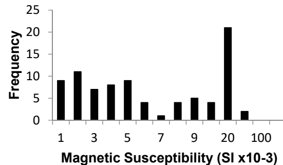
Maraloou Formation n=85
