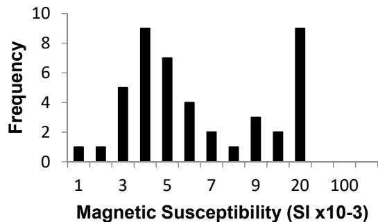
Karalundi Formation n=44
