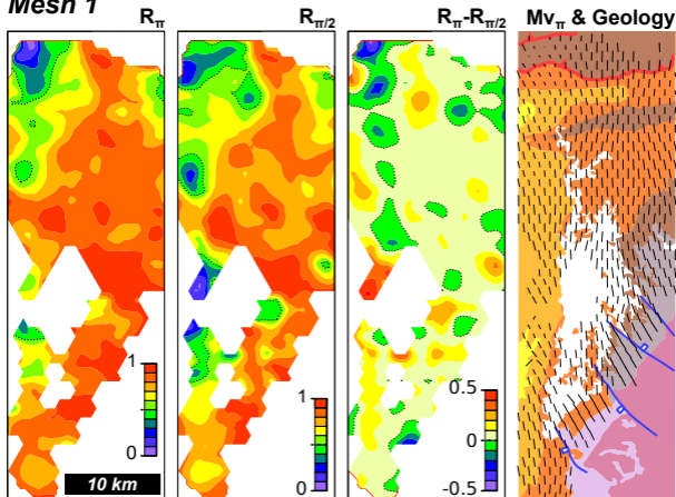
Mesh 1
