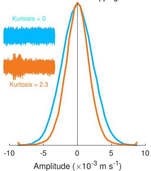
After waveform clipping
