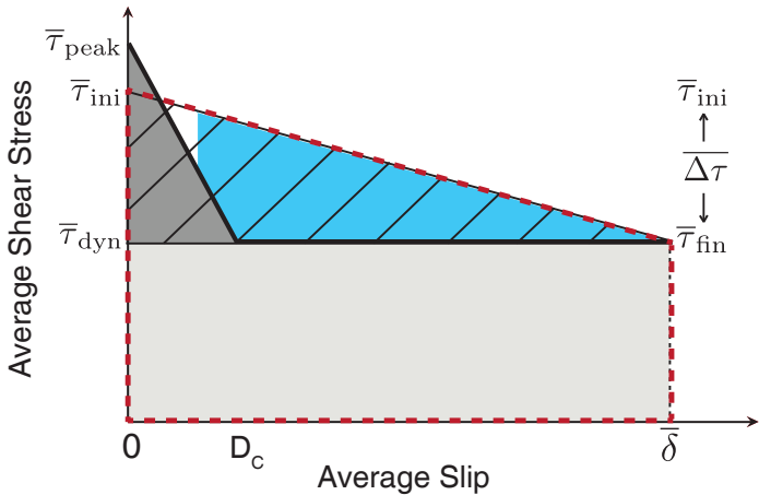
(a) Standard Slip-Weakening Energy Diagram
