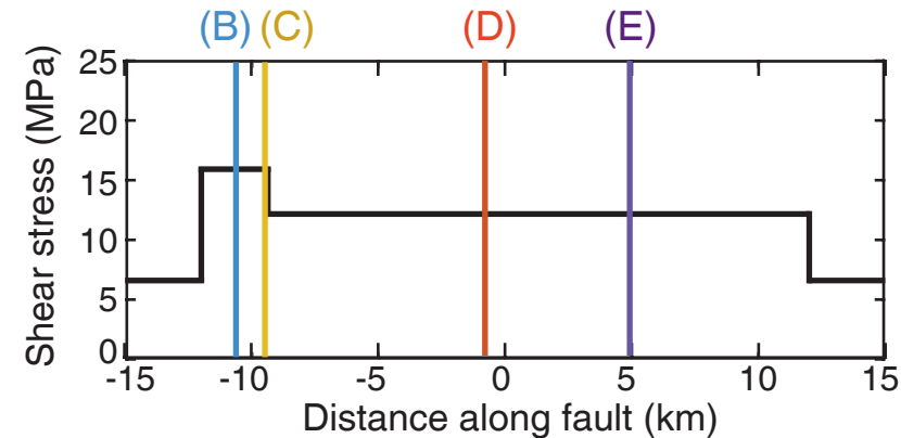
Initial shear stress
