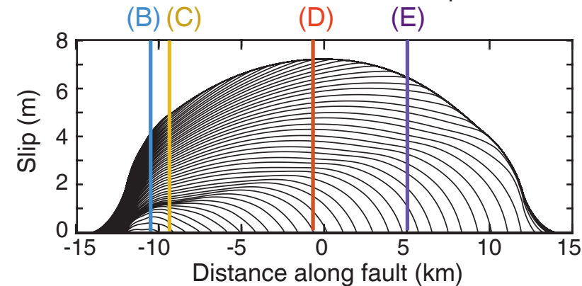
Standard rate-and-state and thermal pressurization
