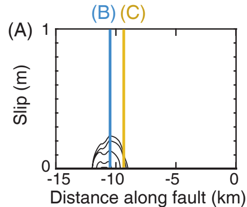
Standard rate-and-state only
