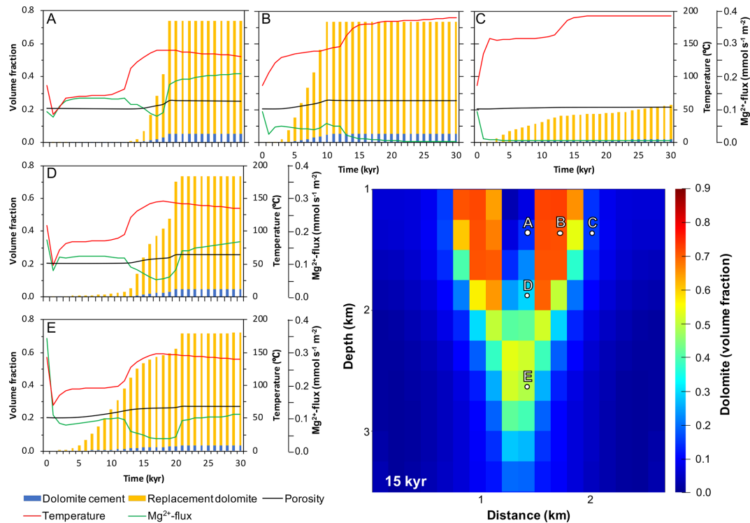
Figure 6. Dolomitisation, \text{Mg}^{2+} -flux, temperature, and porosity change in the FDZ, at locations vertically along the descending flow path (A–E) and laterally with distance from the core (A–B–C). Note how replacement dolomitisation is initially limited by the low temperature in the “up-flow” margin of the dolomite body (A), whereas reactions are limited by \text{Mg}^{2+} -flux in the “down-flow” margin (C).
