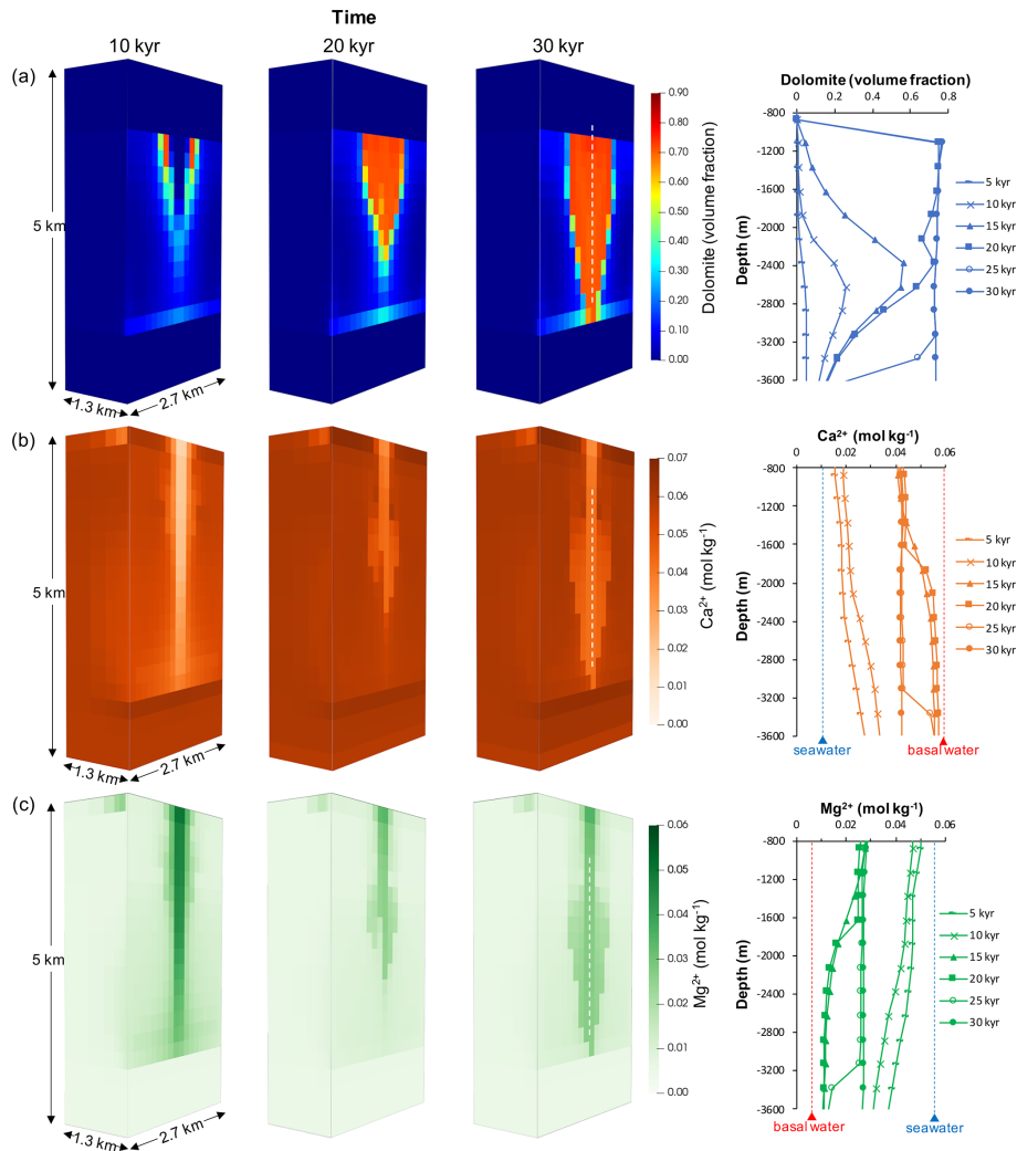
Figure 4. Temporal evolution of the dolomite volume fraction (a), the \text{Ca}^{2+} concentration (b), and the \text{Mg}^{2+} concentration (c) from the 3D baseline simulation, and plots of those changes down the core of the descending limb of the convection cell within the FDZ (white dashed line). \text{Ca}^{2+} is enriched relative to seawater, and \text{Mg}^{2+} is depleted as a result of the replacement of precursor limestone by dolomite. After complete replacement, there is a minor decrease in the concentrations of both \text{Mg}^{2+} and \text{Ca}^{2+} due to dolomite cementation.
