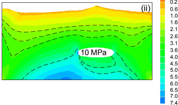
Principal Stress \sigma_1
