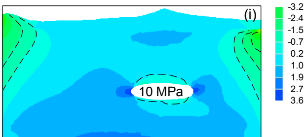
Principal Stress \sigma_3
