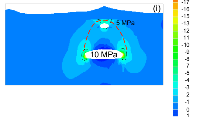
Principal Stress \sigma_1
