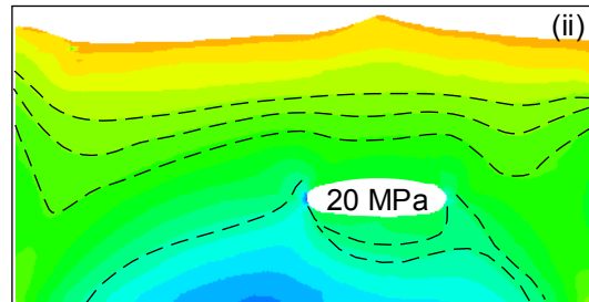
Principal Stress \sigma_1
