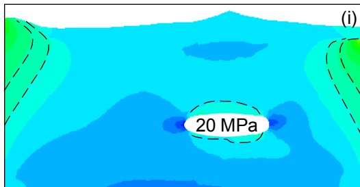
Principal Stress \sigma_3
