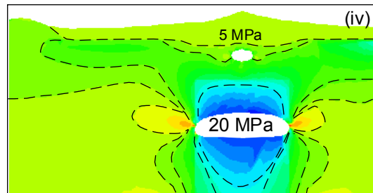
Principal Stress \sigma_1
