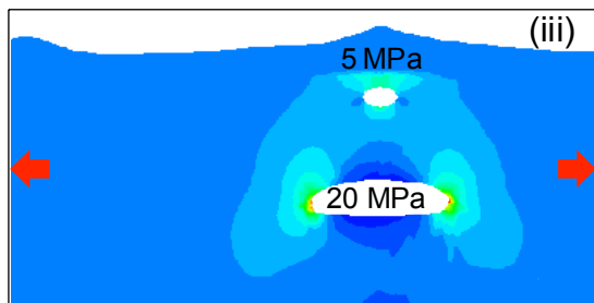
Principal Stress \sigma_3
