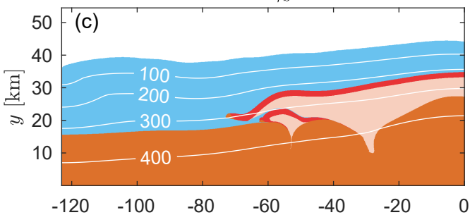
Von Mises plastic basement, C = 75 MPa t = 7.69 Ma - \gamma_b = 38.45 %
