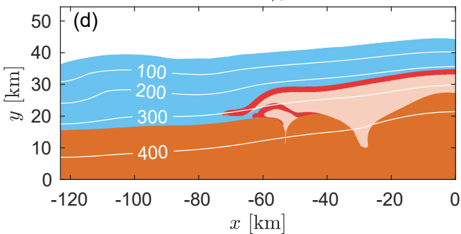
Von Mises plastic basement, C = 100 MPa t = 7.69 Ma - \gamma_b = 38.45 %
