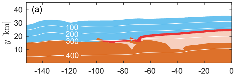
Von Mises plastic basement, C = 25 MPa t = 4.8 Ma - \gamma_b = 24.02 %
