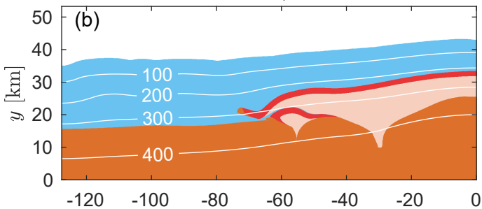
Von Mises plastic basement, C = 50 MPa t = 7.23 Ma - \gamma_b = 36.17 %
