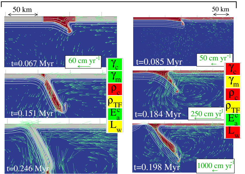
(b) A_o = 5 \text{ Myr} , A_y = 2 \text{ Myr} (c) A_o = 15 \text{ Myr} , A_y = 5 \text{ Myr}
