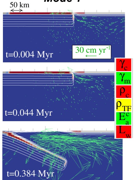
(a) A_o = 50 \text{ Myr} , A_y = 5 \text{ Myr}
