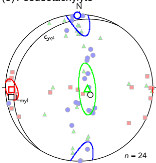
(e) Pseudotachylyte
