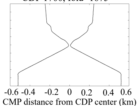
(b) CDP 1700, fold=1675
