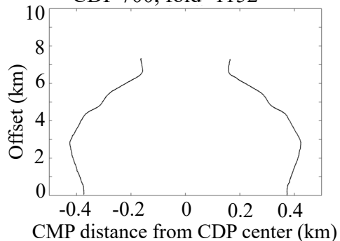
(a) CDP 700, fold=1152
