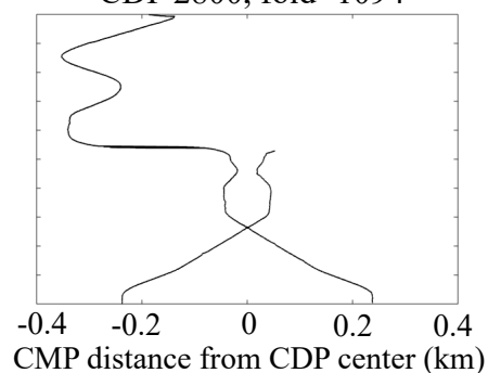
(c) CDP 2800, fold=1094
