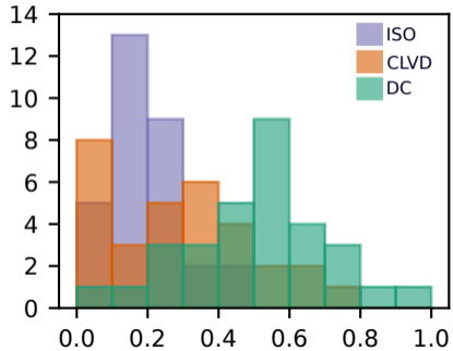
Inversion for full MT
