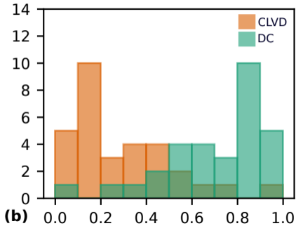
Inversion for deviatoric MT
