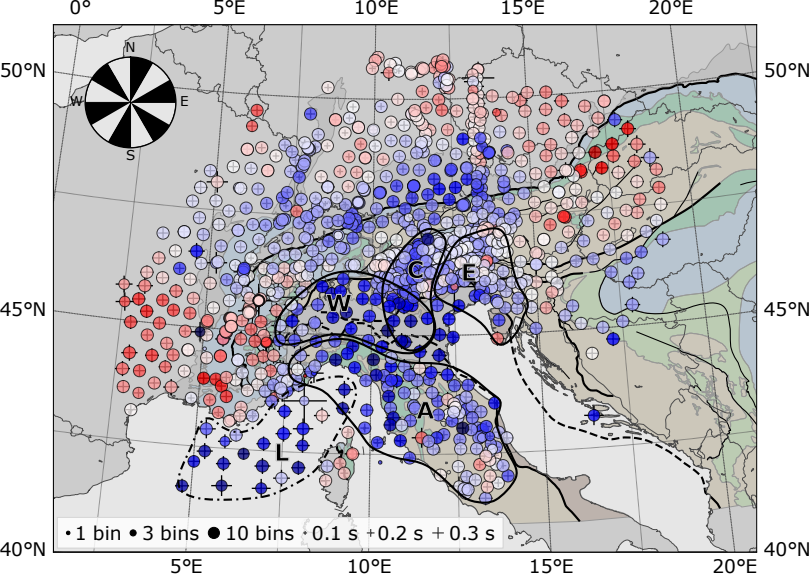
(a) Travel-time residuals of db_{0.1}
