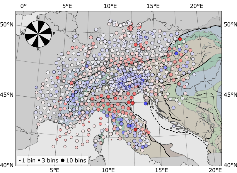
(b) Residual differences db_{0.5} - db_{0.1}
