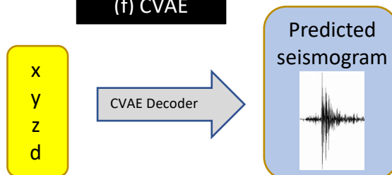
(f) CVAE
