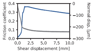
(c) HTB735 (Steady state)
