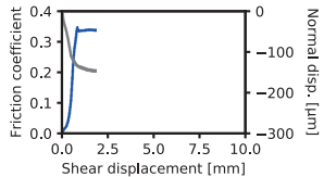
(b) HTB738 (Post-yield)
