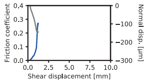
(a) HTB736 (Pre-yield)
