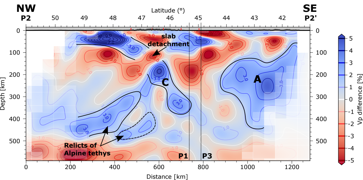
(b) Profile 2: 51.0°N, 6.0°E to 41.0°N, 14.3° E
