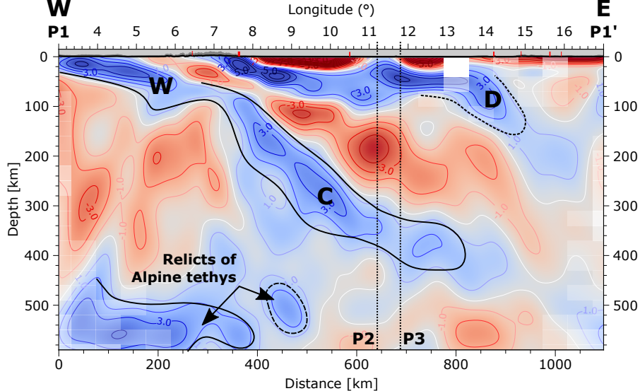
(a) Profile 1: 45.3°N, 3.0°E to 45.0°N, 17.0° E
