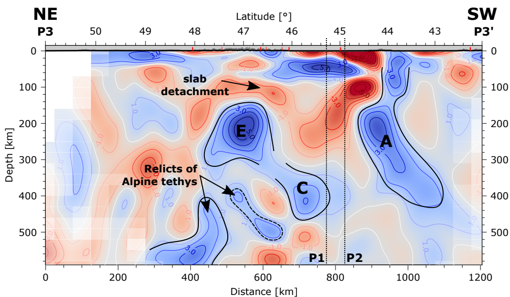
(c) Profile 3: 51.0°N, 17.8°E to 42.0°N, 9.0°E
