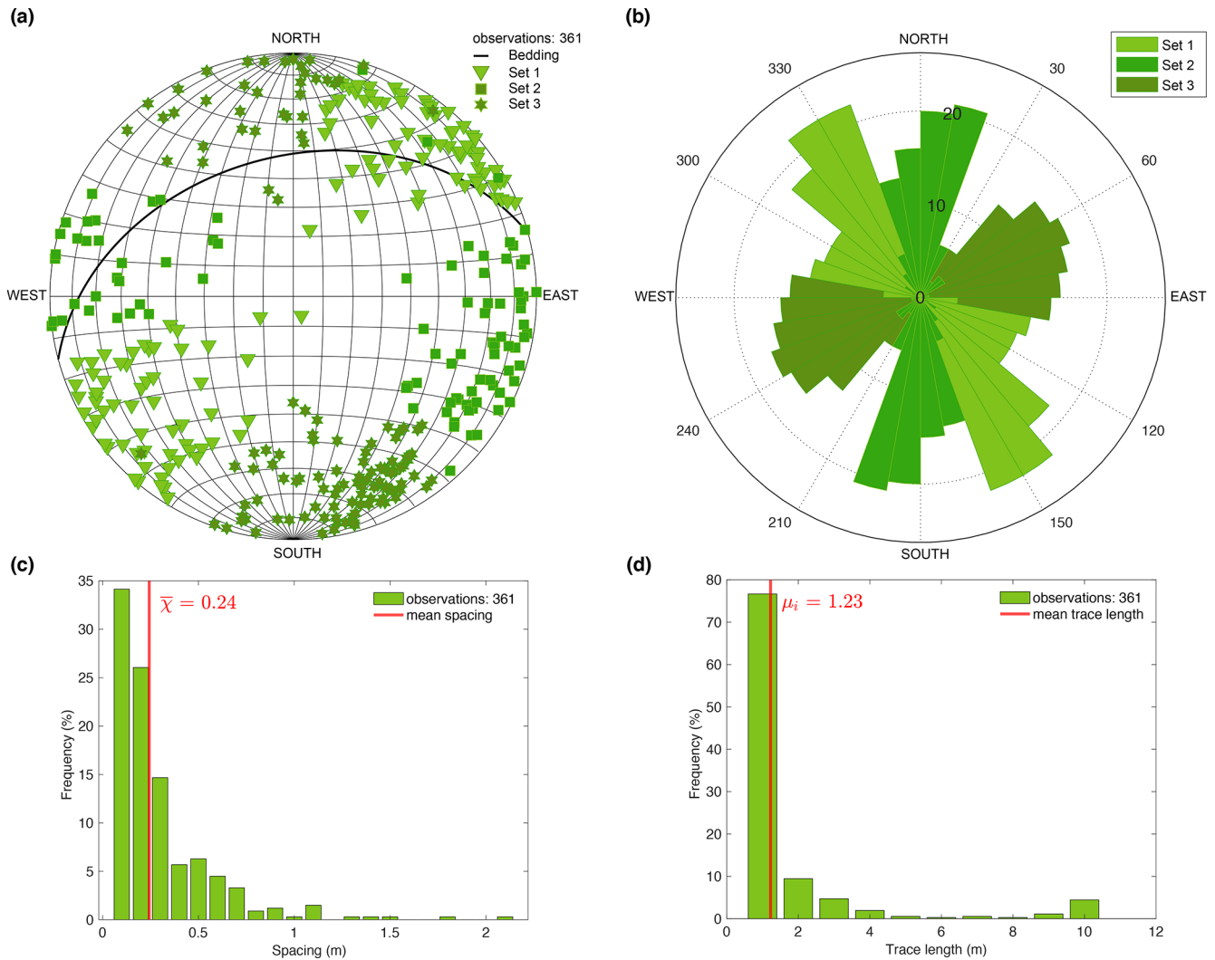
Figure 5. Results of all scanline investigations at the quarry in Hagen-Hohenlimburg: (a) stereogram of measured discontinuity sets and a (b) rose diagram of rotated discontinuity orientations according to the bedding layer in panel (a) for a horizontal position, (c) discontinuity spacing diagram, and (d) discontinuity trace length diagram.
