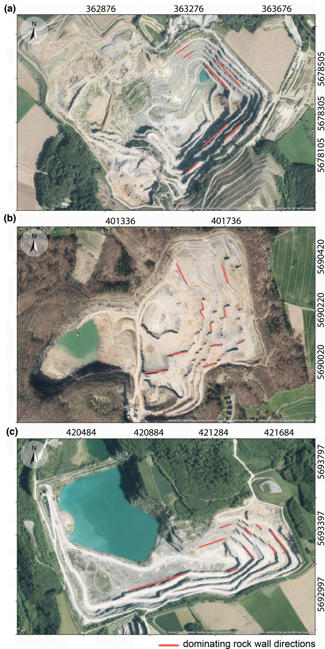
Figure 3. Map view of all three study areas in which scanline surveys were carried out: (a) the Osterholz stone pit, which is operated by Kalkwerke H. Oetelshofen GmbH & Co. KG in Wuppertal; (b) the Oege stone pit, operated by Hohenlimburger Kalkwerke GmbH in Hagen-Hohenlimburg; (c) the Asbeck rock mine, managed by Lhoist Deutschland, Rheinkalk GmbH in Hönnetal. Red lines indicate the predominant rock walls, i.e. the direction of the mining. In each of the three outcrops there were two dominant mining directions, which were approximately perpendicular to each other. This figure was created using ArcGIS® software by Esri (Basemap, World Imagery: http://www.arcgis.com/home/item.html?id=10df2279f9684e4a9f6a7f08febac2a9 , last access: 24 March 2020). © ArcGIS and ArcMap™ are the intellectual property of Esri and are used herein under license. © Esri. All rights reserved. For more information about Esri™ software, please visit http://www.esri.com (last access: 24 March 2020).
