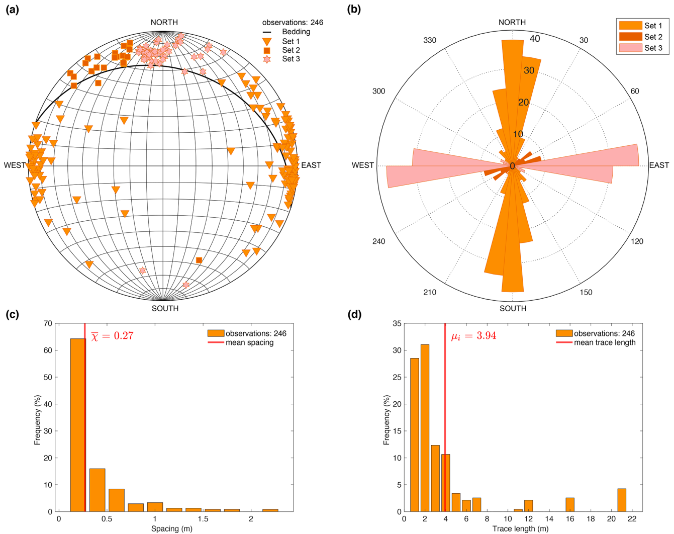
Figure 6. Results of all scanline investigations at the quarry in Hönnetal: (a) stereogram of measured discontinuity sets and a (b) rose diagram of rotated discontinuity orientations according to the bedding layer in panel (a) to a horizontal position, (c) discontinuity spacing diagram, and (d) discontinuity trace length diagram.
