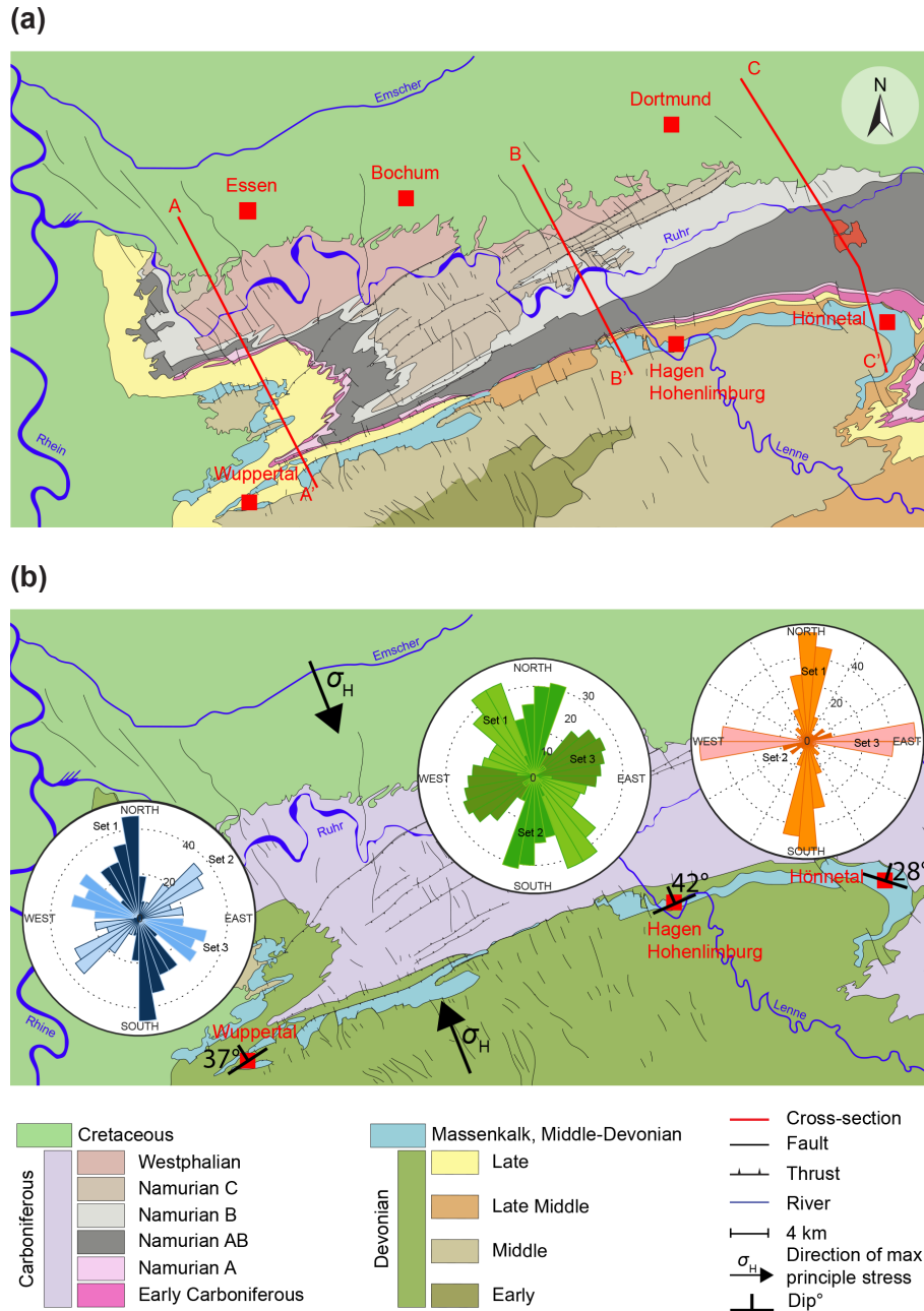
Figure 1. (a) Simplified geological map of the Rhine-Ruhr metropolitan area, Germany (modified from Jansen et al., 1986; Drozdowski et al., 2007). Here, three stone pits have been chosen for field surveys: Osterholz (Wuppertal), Oege (Hagen), and Asbeck (Hönnetal), which are part of the Devonian Reef Complex (Massenkalk). The red lines indicate the three geological cross sections as shown in Fig. 2. In panel (b), the geological map from panel (a) was further simplified, and in addition the rose diagrams of the discontinuity sets as measured by scanline investigations at the quarries in Wuppertal (blue), Hagen-Hohenlimburg (green), and Hönnetal (orange) are added (for more detail, see Figs. 4 to 6). The arrows indicate the direction of maximum horizontal stress \sigma_H according to the World Stress Map (Heidbach et al., 2016). The specific directions and angles of incidence of the investigated, exposed limestone layers are also shown in panel (b).
