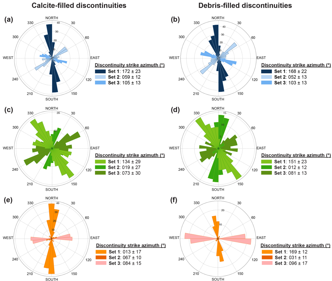
Figure 7. Rose diagrams of measured discontinuity sets at the quarries (a, b) Wuppertal, (c, d) Hagen-Hohenlimburg, and (e, f) Hönnetal as a function of their discontinuity filling, i.e. whether the discontinuities are filled with (a, c, e) calcite or (b, d, f) debris. The discontinuity strike azimuths given next to the figures correspond to the arithmetic mean values and the corresponding standard deviations.
