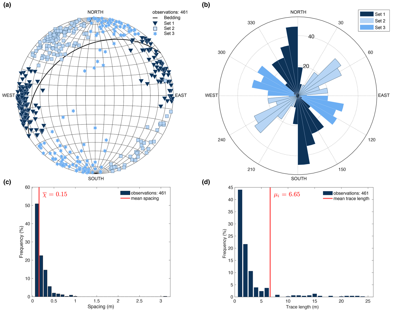
Figure 4. Results of all scanline investigations at the quarry in Wuppertal: (a) stereogram of measured discontinuity sets and a (b) rose diagram of rotated discontinuity orientations according to the bedding layer in panel (a) for a horizontal position, (c) discontinuity spacing diagram, and (d) discontinuity trace length diagram.
