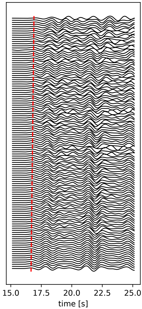
N component
