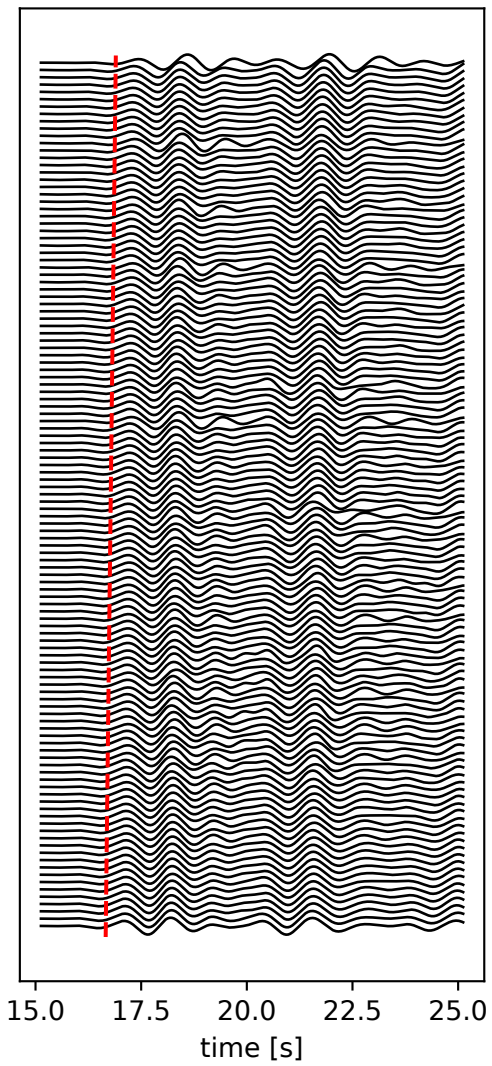
Z component
