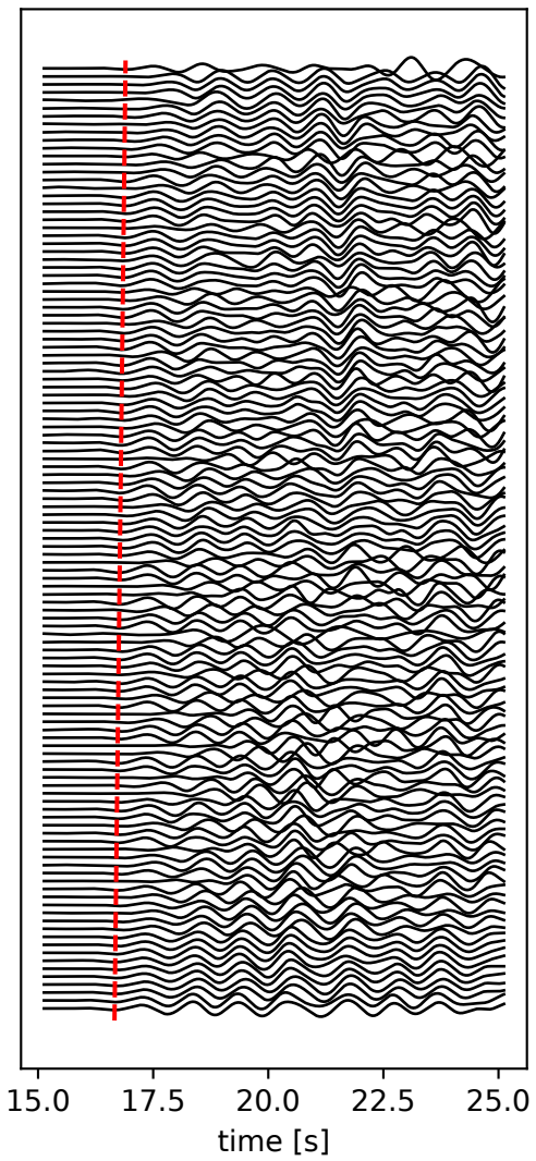
E component
