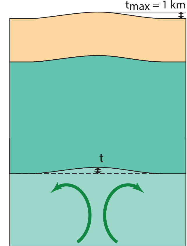
(e) Mantle upwelling Before erosion: dynamic topography
