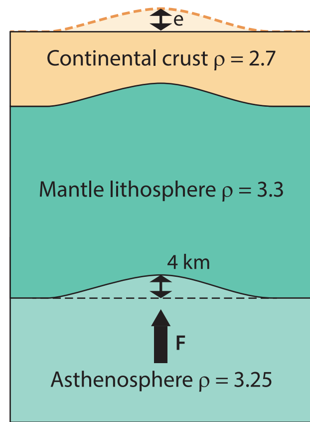
(a) Lithospheric uplift, generic case
