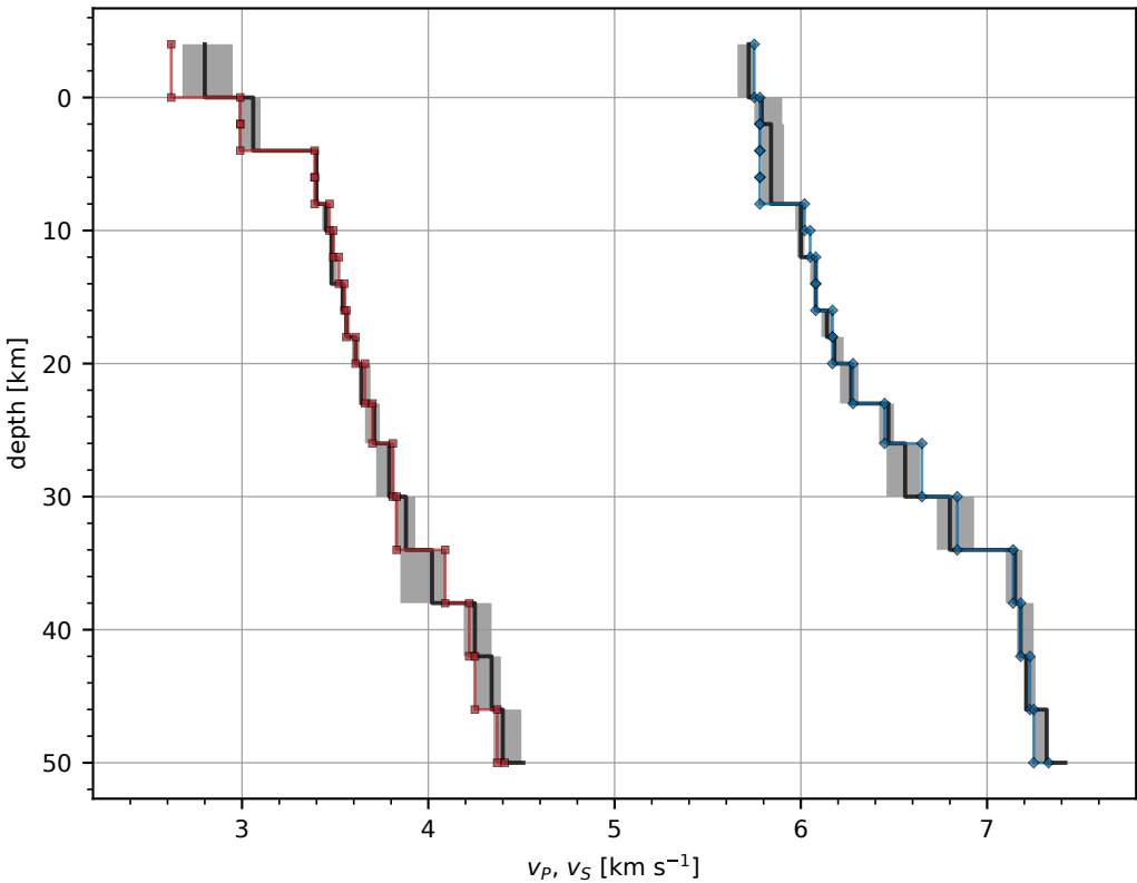
Selected 1-D P and S model with final velocity distribution
