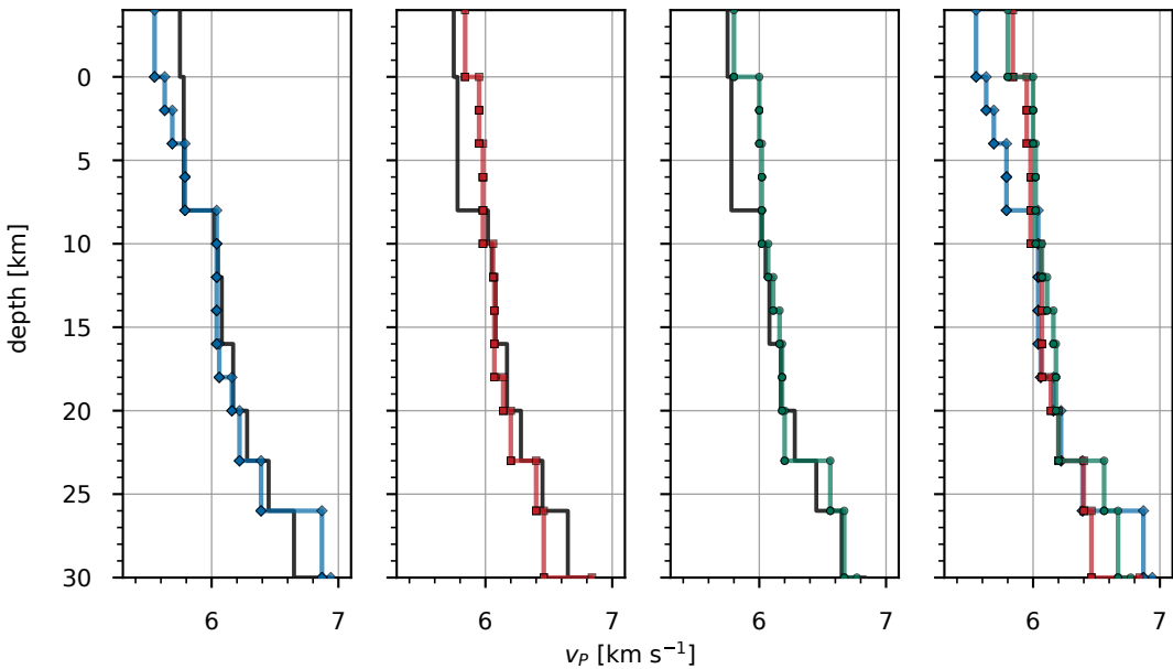
Comparison of selected 1-D velocity models by subregion (P velocity)
