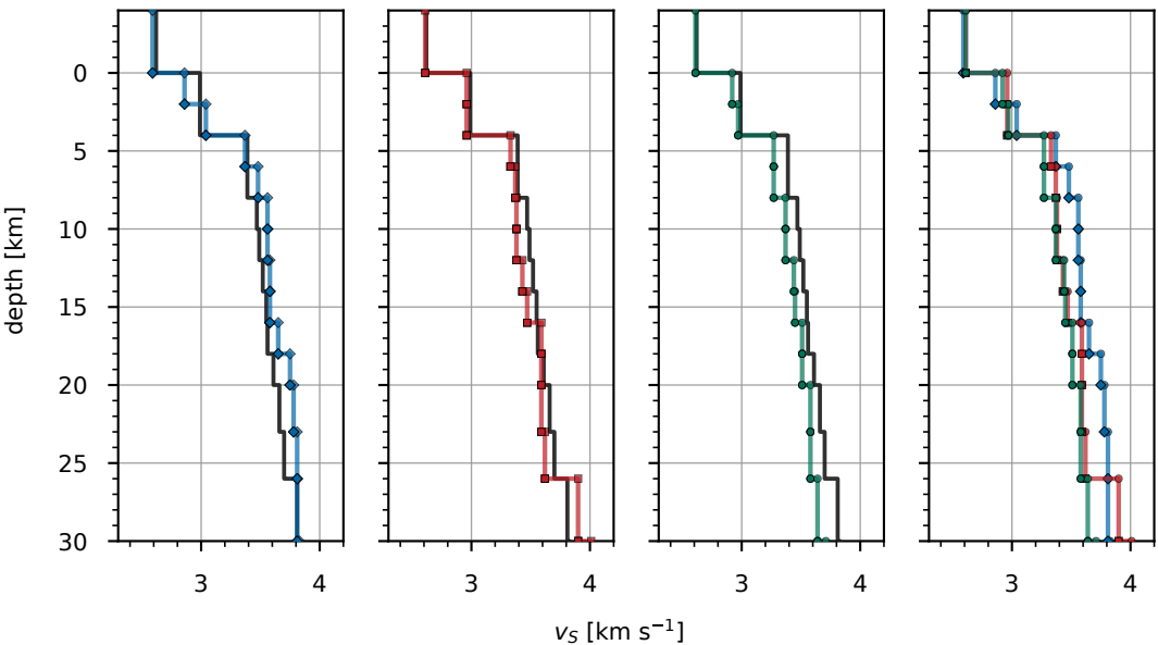
Comparison of selected 1-D velocity models by subregion (S velocity)
