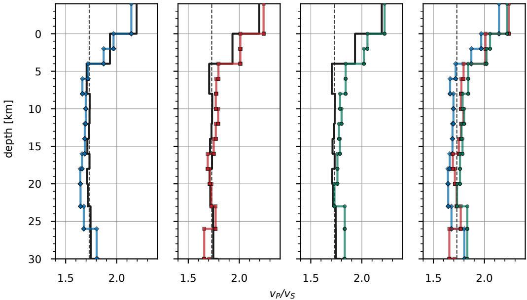
Comparison of v_P/v_S by subregion
