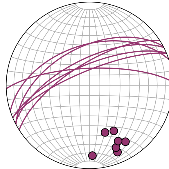
Fault zone
