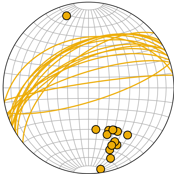
Mylonite
