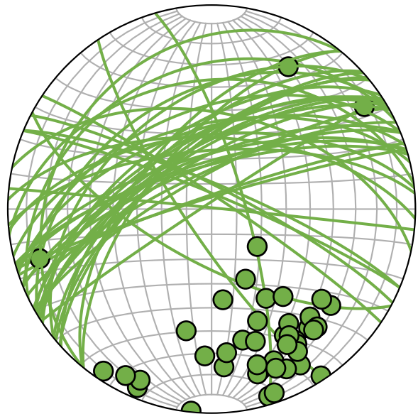
Rugose micaceous fracture
