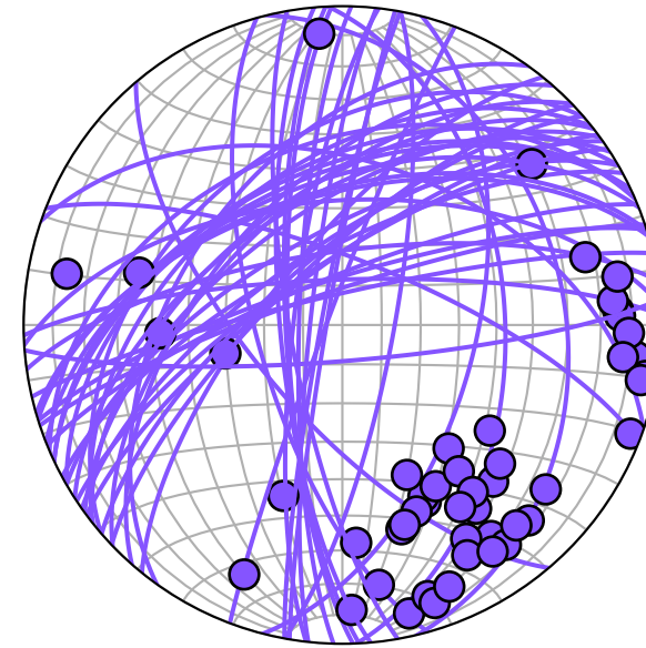
Shear fracture (split)
