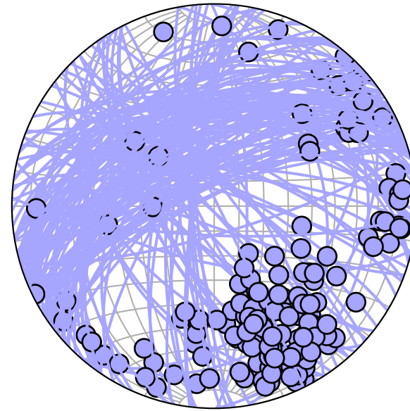
Shear fracture (closed)
