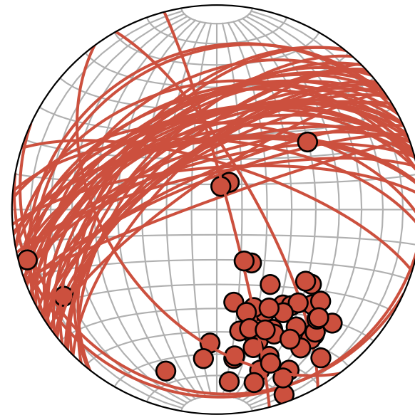
Rugose fracture (open)
