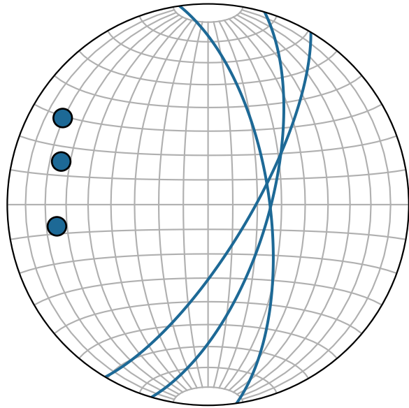
Biotite alignment
