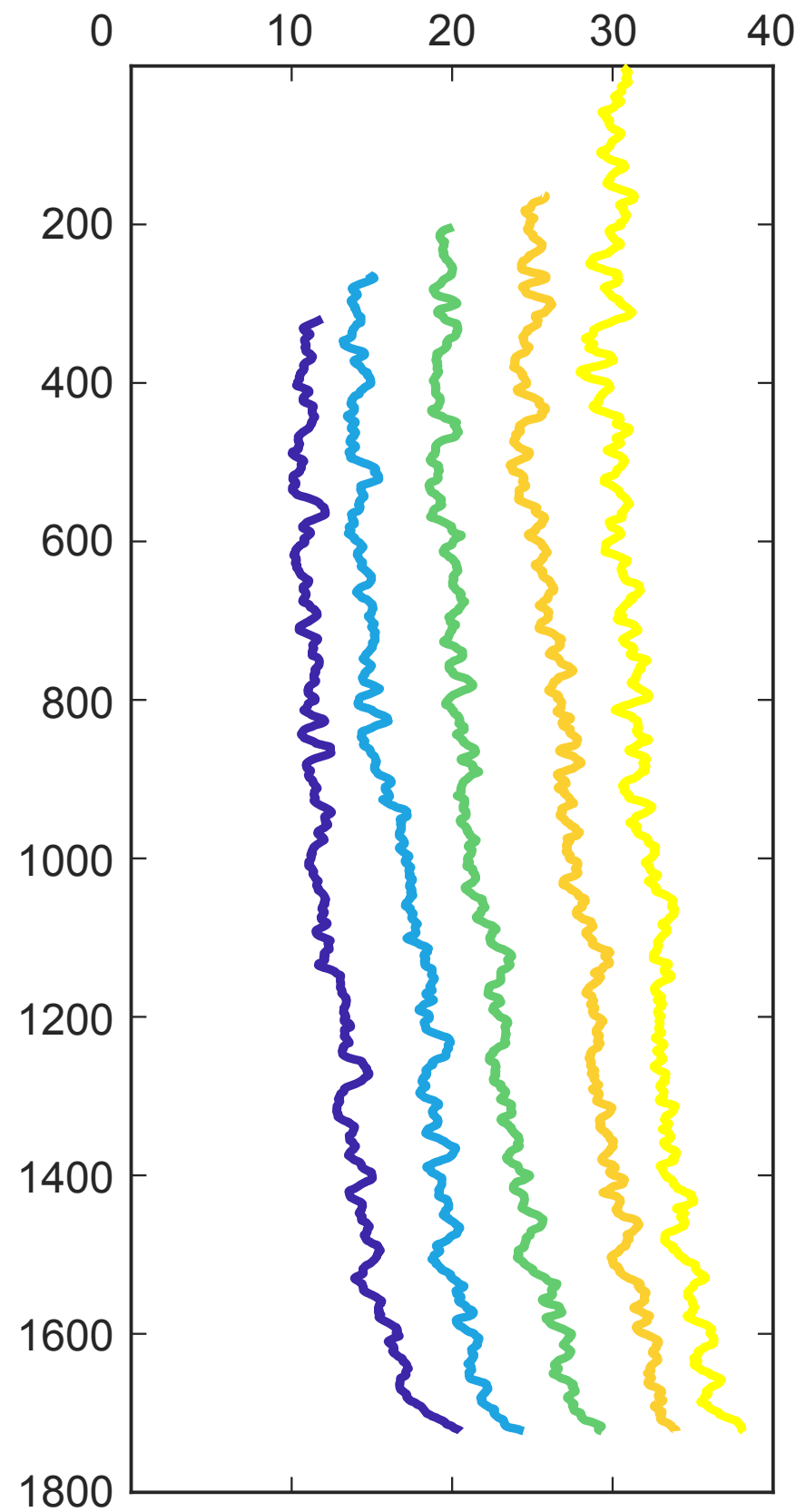
(c) Porosity [%]
