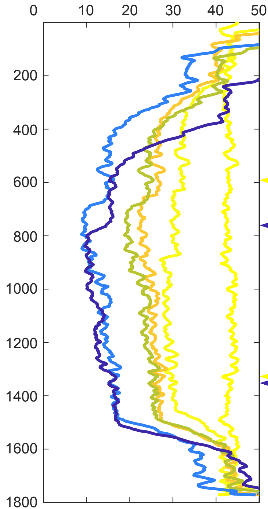
(a) Porosity [%]
