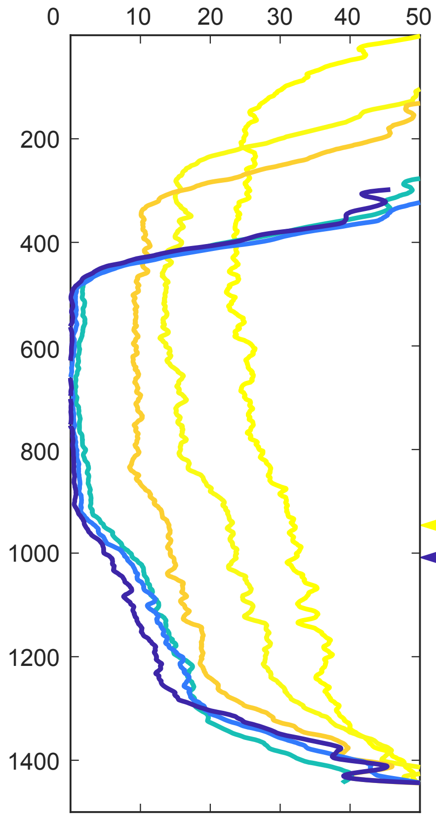
(b) Porosity [%]
