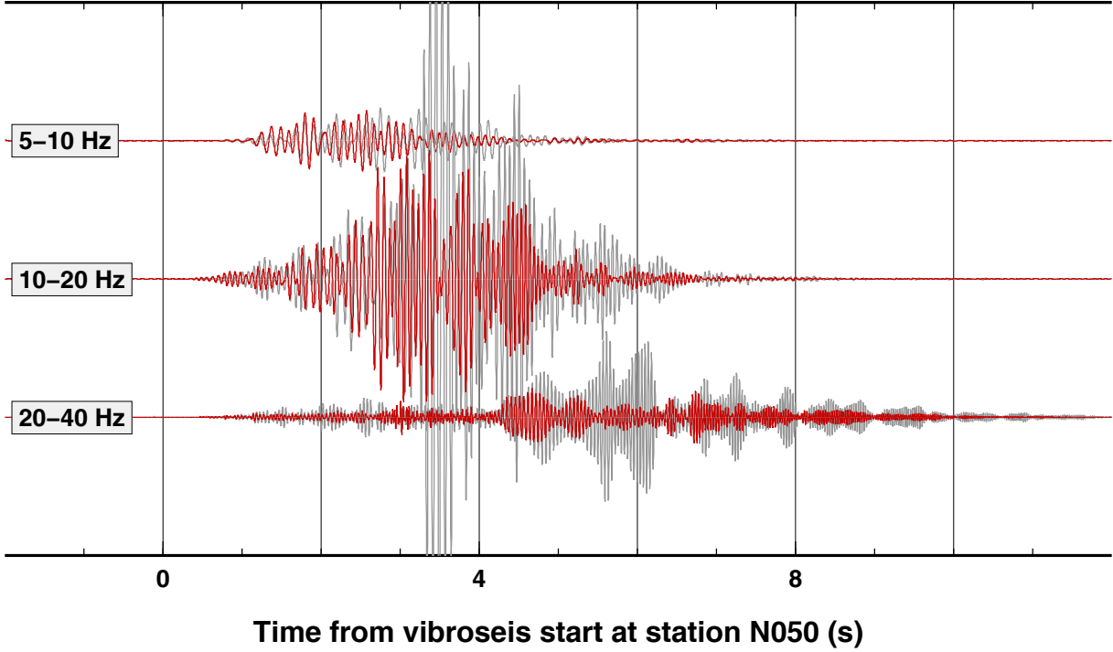
(b) Recordings of vibroseis sweep T49 at node: N050 (grey lines) and channel: 5479 (red lines)
