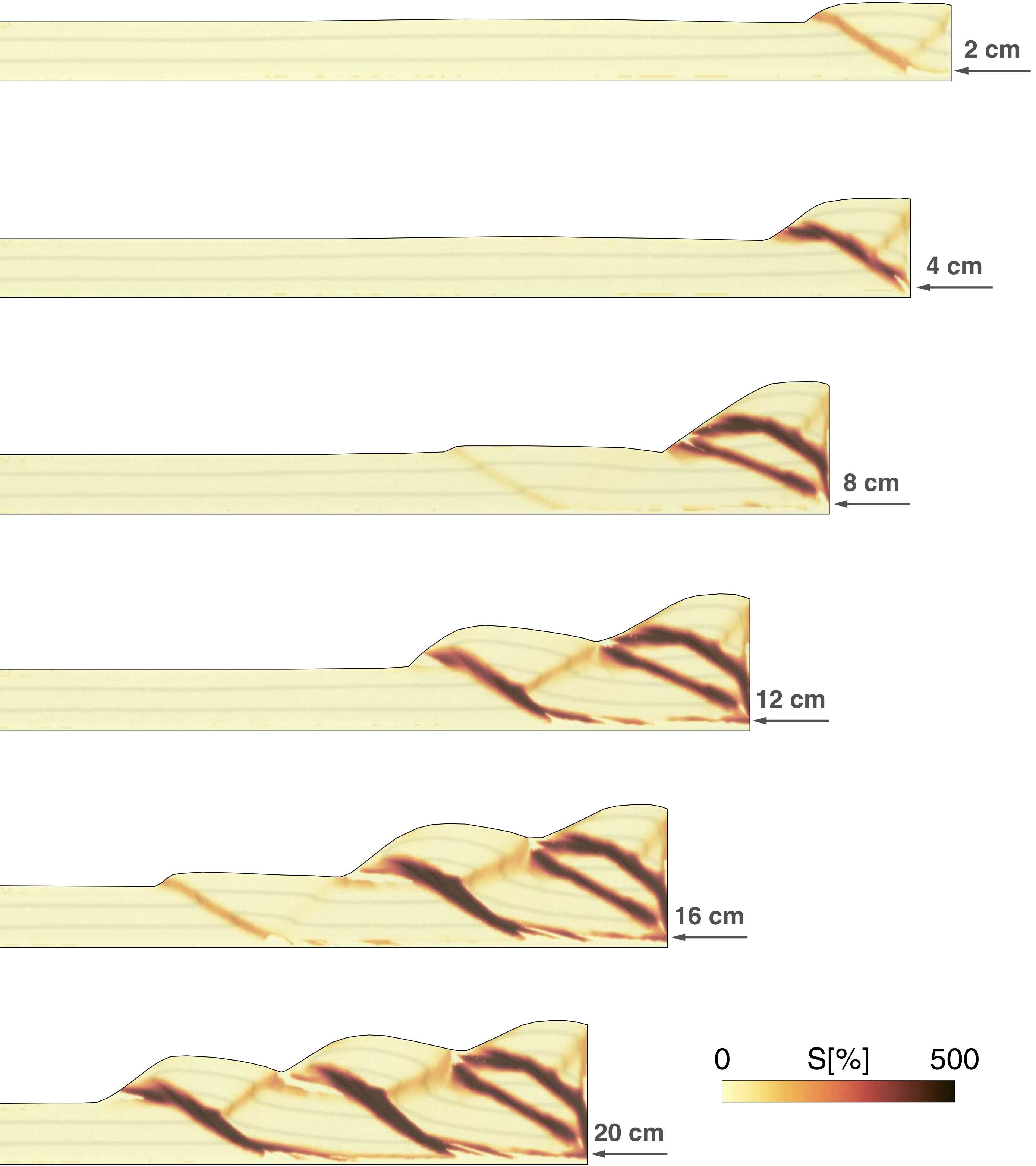
(c) Cumulative strain
