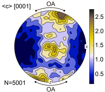
(a) Quartz c-axes projected onto a Schmidt net
