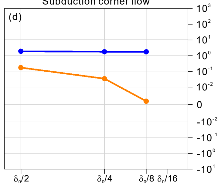
Subduction corner flow
