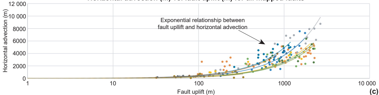
Horizontal advection (m) vs. fault uplift (m) for all mapped faults
