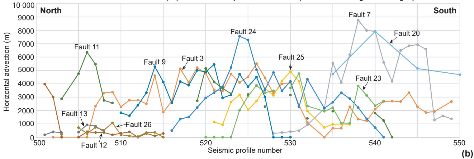
Horizontal advection (m) vs. Seismic profile number (distance along the margin)
