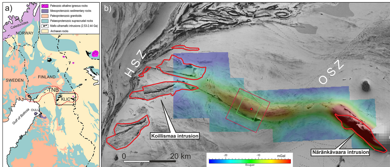
Figure 1. (a) Simplified geological map of the Fennoscandian Shield (modified from Karinen, 2010); KLIC: Koillismaa–Näränkävää Layered Intrusion Complex, TNB: Tornio–Näränkävää Belt; (b) location of the study area with the composite image of the magnetic anomaly (Aeromagnetic anomaly map of Finland © Geological Survey of Finland 2016), Bouguer gravity anomaly (Salmirinne and Iljina, 2003) and simplified bedrock geology (Bedrock of Finland 1 : 1 000 000 © Geological Survey of Finland 2016) maps. Red dot marks the Koillismaa drillhole, rectangles mark the extend of the SEEMS DEEP 3D seismic survey (green) and the Common Earth Model area (red); HSZ: Hirvaskoski Shear Zone, OSZ: Oulujärvi Shear Zone. Total Magnetic Intensity shading from low (white) to high values (black).
