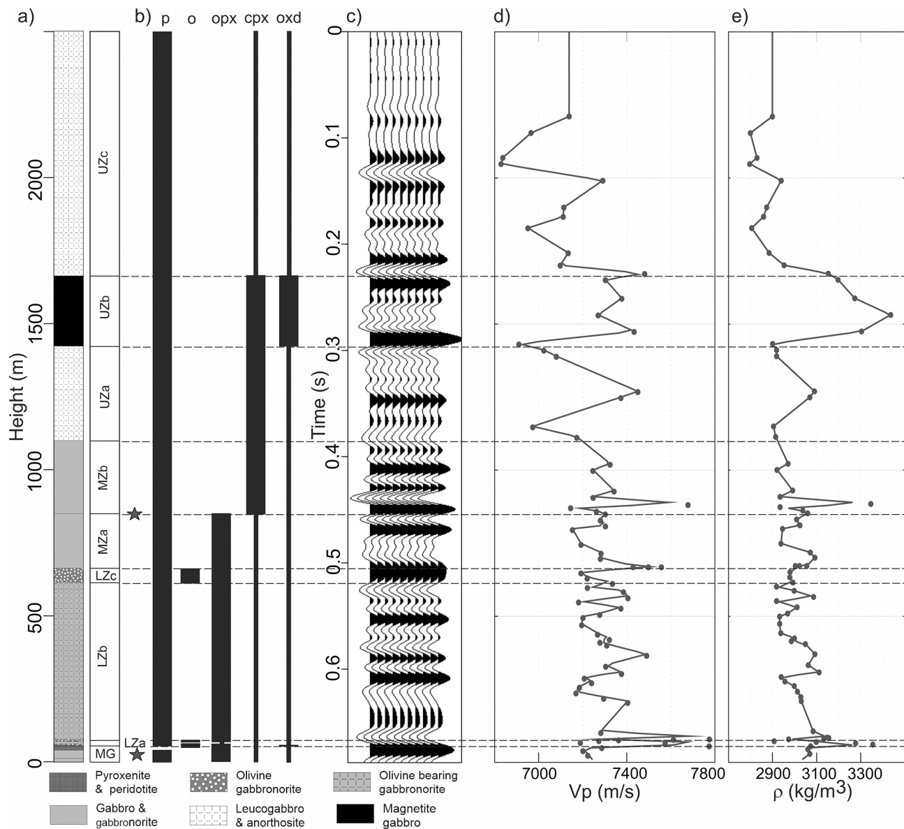
Figure 3. (a) Representative stratigraphic section of KLIC based on the profile across the Porttivaara block (Karinen, 2010); (b) In the sequence thick vertical lines indicate cumulus minerals and thin vertical lines indicate intercumulus minerals (p-plagioclase, o: olivine, opx: orthopyroxene, cpx: clinopyroxene, oxd: Fe-Ti oxides); stars denote occurrence of sulphide mineralisation (up to 3 %); (c) corresponding filtered (up to 62.5 Hz) zero-offset reflection coefficient series based on the velocity and density calculated from modal mineralogy; (d) calculated velocity log; (e) calculated density log. Points represent samples and the lines are the interpolated values.
