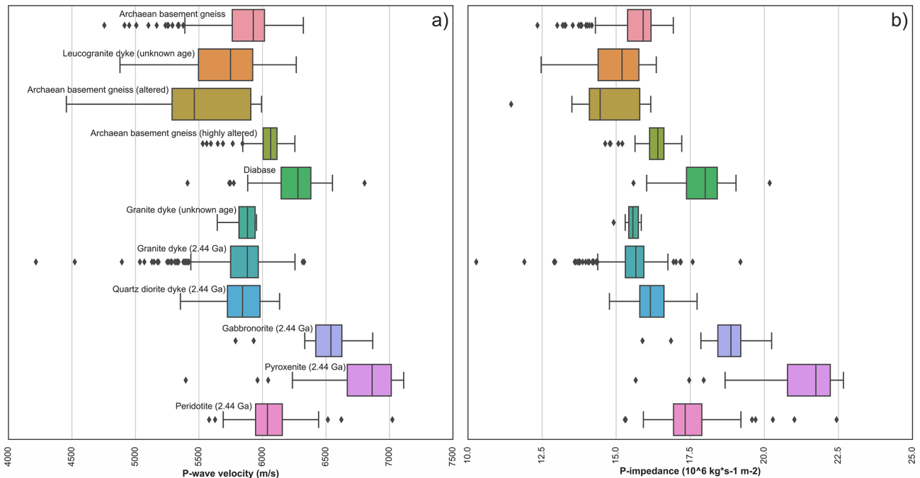
Figure 2. (a) Box-and-whisker plot of the measured P-wave velocity using core samples from the Koillismaa deep drillhole grouped by the rocktype and ordered approximately by depth. The 2.44 Ga age is related to the intrusion. (b) Corresponding acoustic impedance plot based on the co-located velocity and density measurements.
