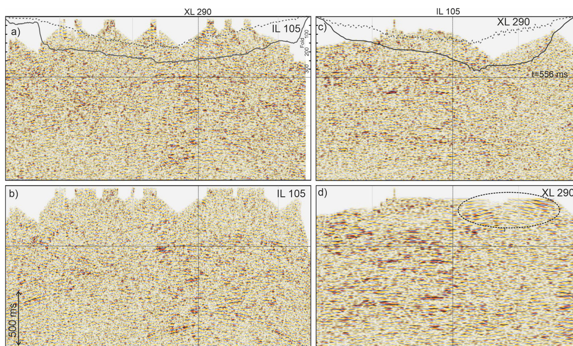
Figure 6. Inline and crossline sections through the stack volumes without (a, c) and with (b, d) pre-stack 5D interpolation. Stacking fold is plotted at the top: normal stack – dashed line, interpolated stack – solid line.
