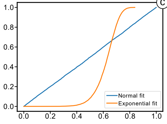
Empirical cumulative of the CDF for the fitted distributions
