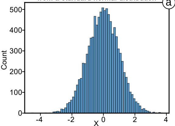
Frequency of 10000 random samples from a standard normal distribution
