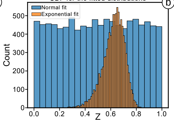
Frequency histogram of the CDF for the fitted distributions
