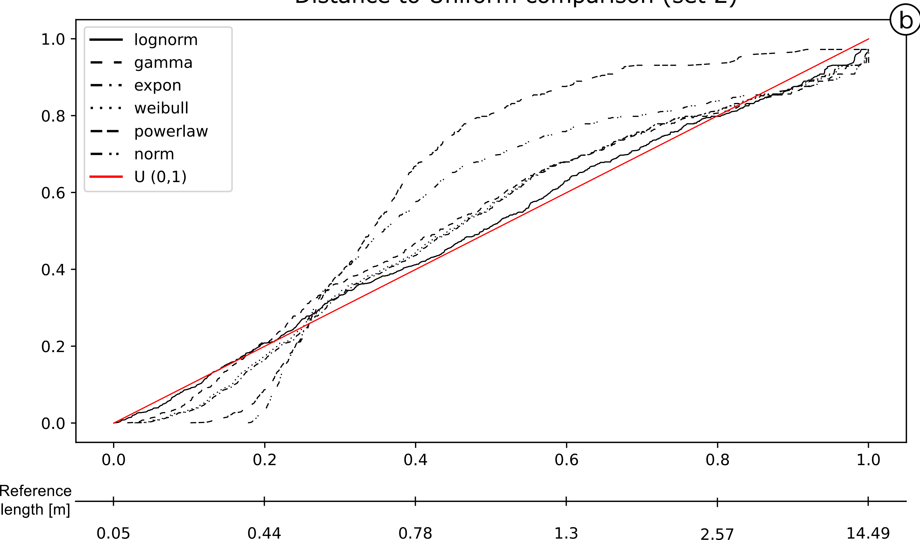
Distance to Uniform comparison (set 2)
