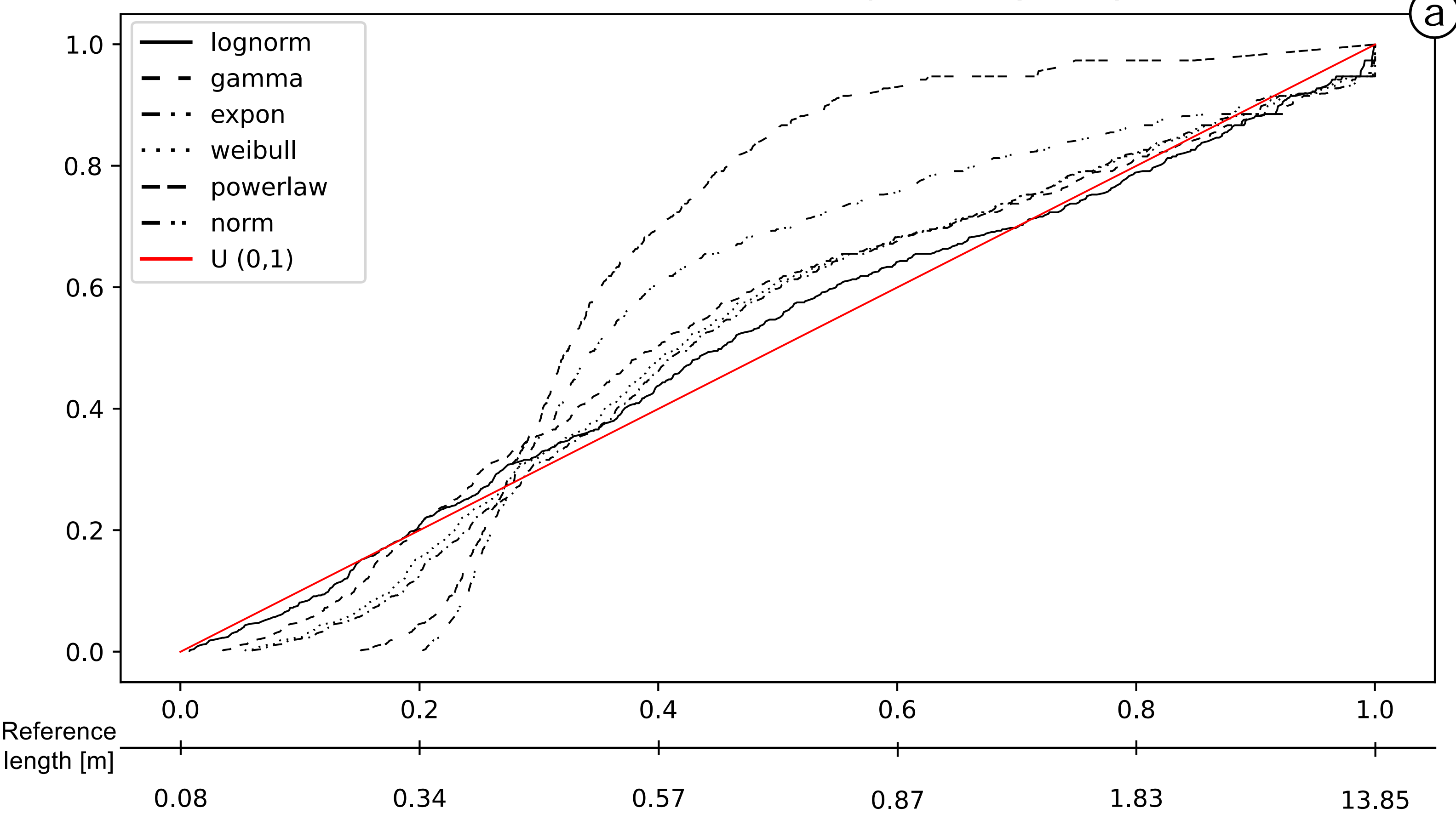
Distance to Uniform comparison (set 1)
