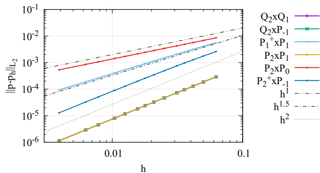
(b) structured mesh
