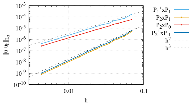
(c) unstructured mesh
