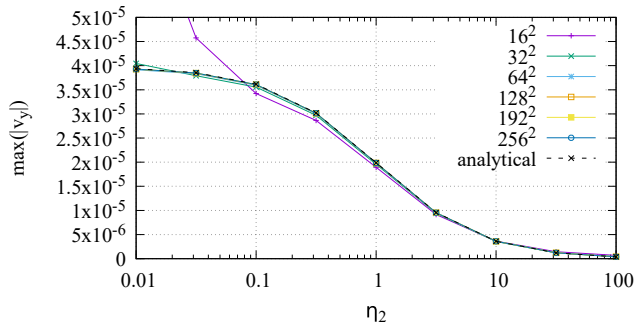
Q_2 \times P_1
