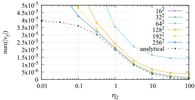
P_2 \times P_0
