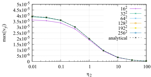
P_1^+ \times P_1
