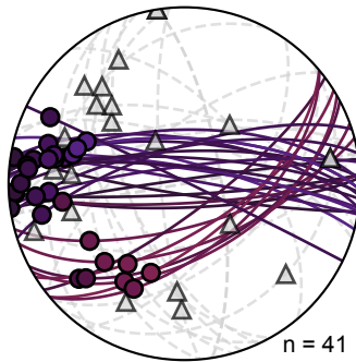
(c) Subdomain C Wildhorn
