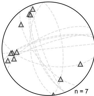
(b) Subdomain B Diablerets
