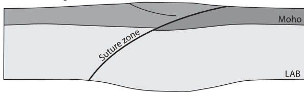
(a) Small, cold orogen
