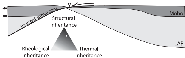
(c) Suture reactivation dominates rift
